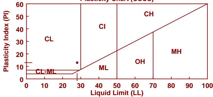
Plasticity Chart (USCS)
